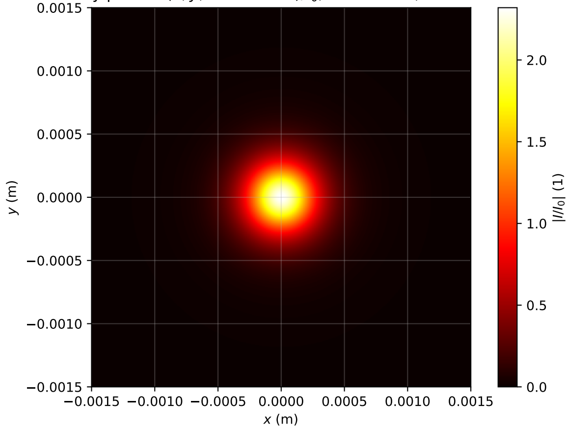
Intensity profile I(x, y, z = 2.388m)/I_0 , Pin=1.0Pcr, artificial time
